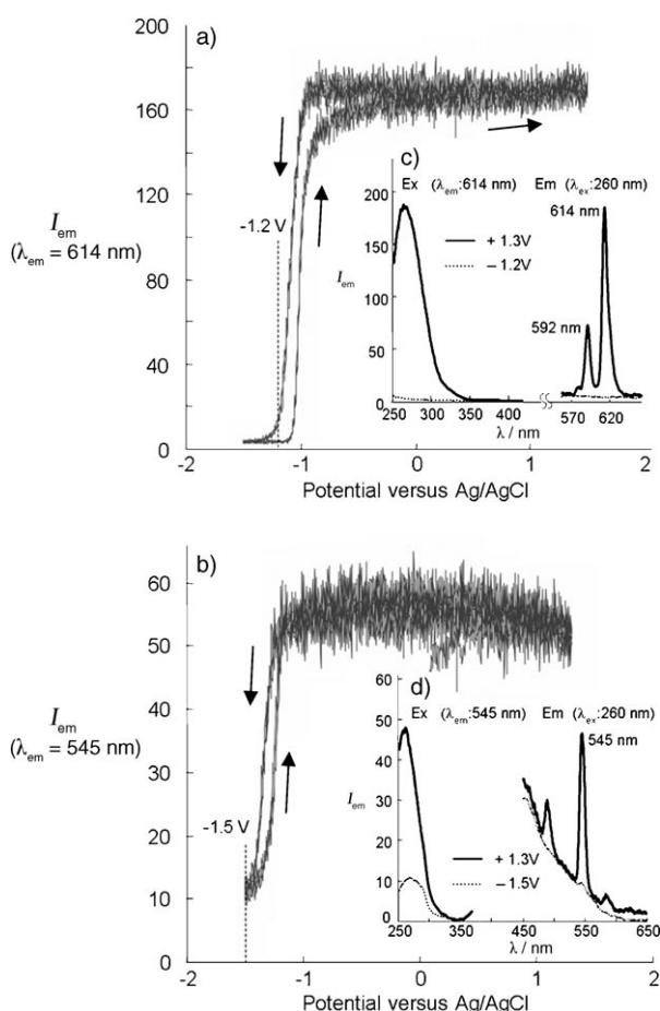
Figure 2. Emission intensity as a function of applied potential (sweep rate: 20 mV min -1 ) for a) the TiO/Eu film ( \lambda_{ex} : 260 nm, \lambda_{em} : 614 nm) and b) the NbO/Tb film ( \lambda_{ex} : 260 nm, \lambda_{em} : 545 nm), as well as photoluminescence spectra recorded at different applied potentials for c) the TiO/Eu film and d) the NbO/Tb film. Em = emission, Ex = excitation.
